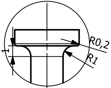
DETAIL C SCALE 5:1
